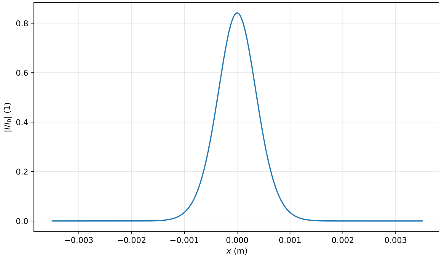
Intensity profile I(x, y = 0, z = 1.353m)/I_0 , P_{in}=0.3P_{cr} , artificial time
